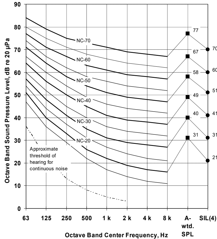
Figure 6.6-1—NC Curves
