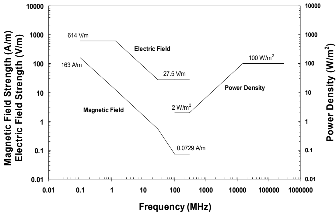
Figure 6.8-1—RF Electromagnetic Field Exposure Limits
