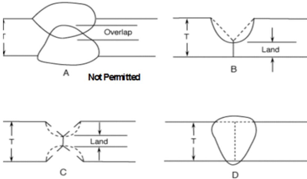
Figure 2—Welding Techniques
