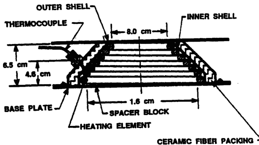
FIGURE 4. Conical Heater
